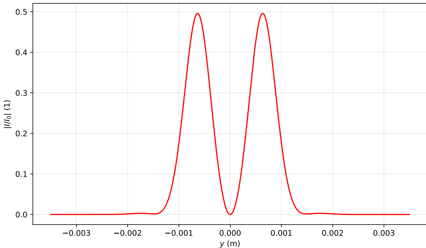
Intensity profile I(x=0, y, z=1.513)/I_0 , P_{in}=3.0P_{cr} , artificial time
